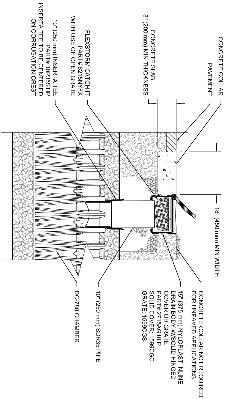
DC-780 10" INSPECTION PORT DETAIL NTS
